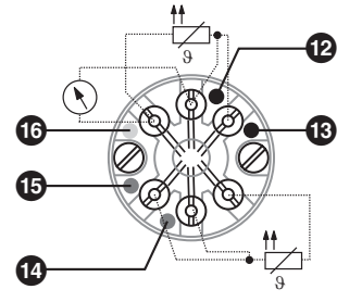
TRG 5-54 (2 x Pt 100)
