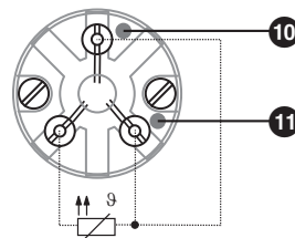
TRG 5-53 (1 x Pt 100) TRG 5-55 TRG 5-57
